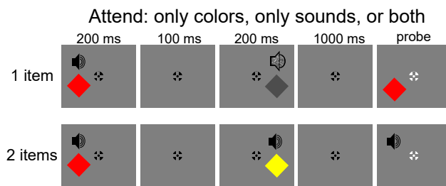
Figure 1. Experiment 1 task
